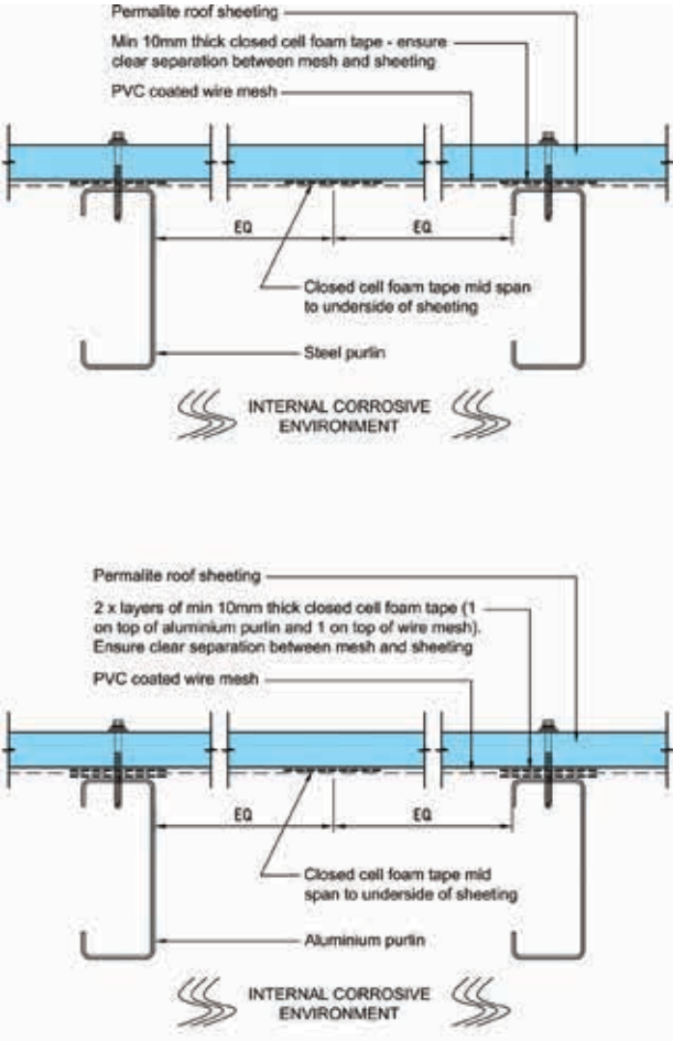
Figure 5.2: Typical wire mesh separation methodology when corrosive environment is internal
