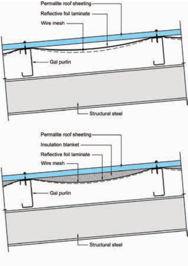
Figure 5.1: Typical roof insulation with foil or combined foil and blanket insulation
