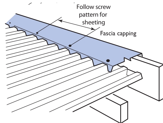
Figure 4.8: Parapet flashing
