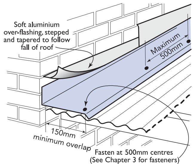
Figure 4.5: Longitudinal flashing
