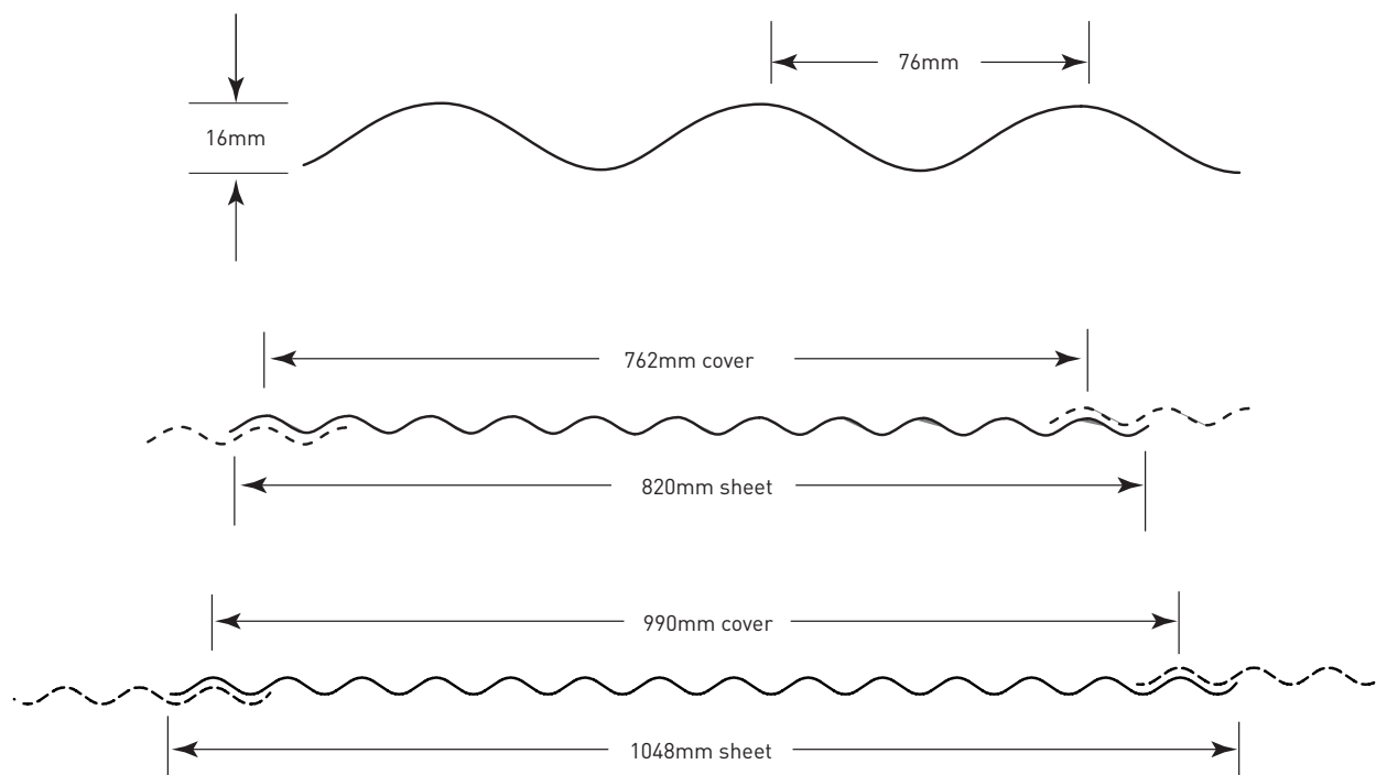
Figure 2.5: PERMALITE WAVELINE® Profile
