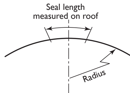
Figure 2.9: Seal length calculation
