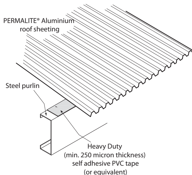
Figure 2.6: Intermaterial preparation measures
